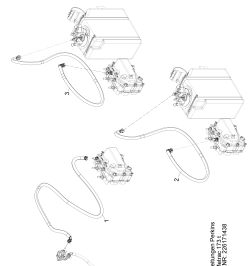
DEF - AdBlue Metrac H95 / Perkins
